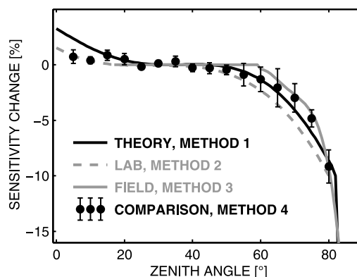
Figure 2. Sensitivity change of Brewer relative to SZA = 35°; black symbols show the mean and expanded standard error of the differences between the Brewer #086 and the Bentham for 5° SZA intervals; lines are fitted splines from Figure 1.
