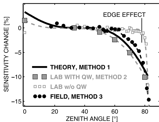
Figure 1. Change in Brewer spectrophotometer sensitivity as a function of SZA from theoretical calculations, laboratory measurements, and field measurements with and without the quartz window. The derived changes are normalized to SZA = 35°. Dashed lines are fitted splines.
