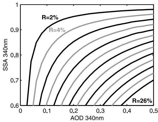
Figure 3. SSA as a function of AOD at 340 nm at SZA = 60° for given reduction R of global irradiance E ; R = 100 \cdot (E_{SSA} = 1 - E_{GLO,SSA}) / E_{SSA} = 1 . The curves correspond to 2% increments of R from R = 2\% to R = 26\% .
